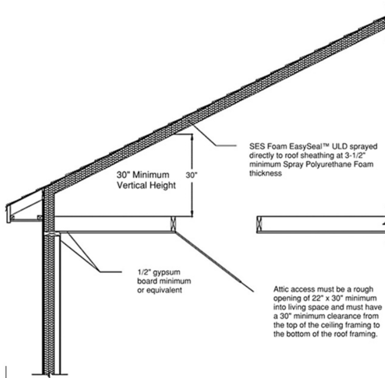
Figure 3. Attic Access
